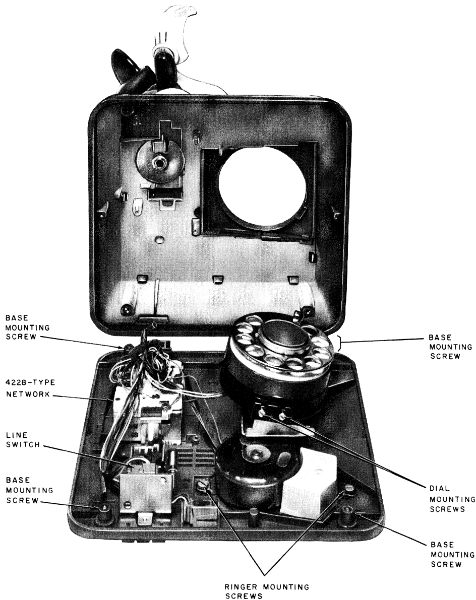
Fig. 2—881B109 Telephone Set With Base
